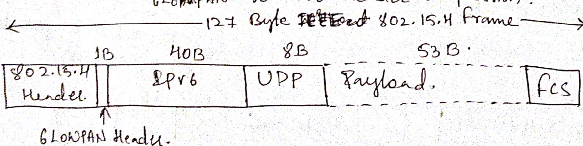
Figure (c) :- 6LOWPAN Header Compression :-
